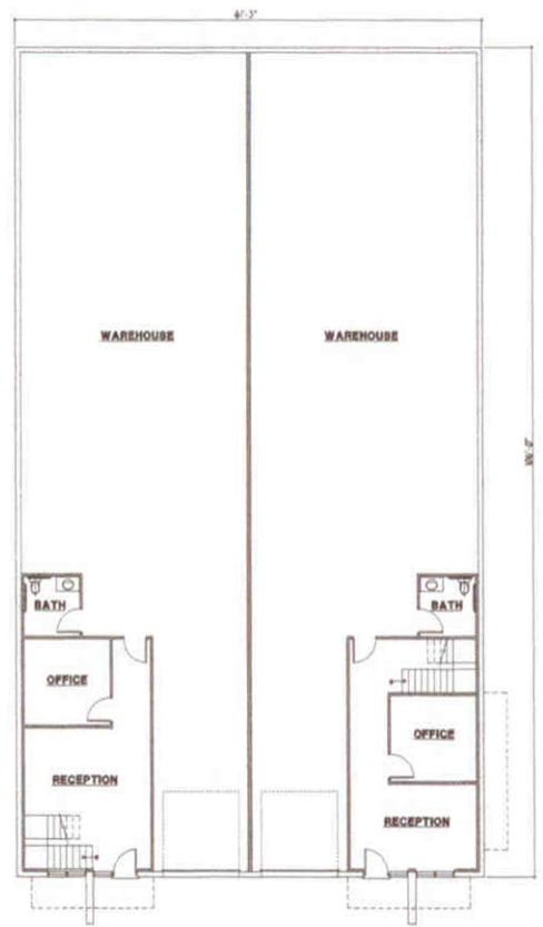
FRIST FLOOR PLAN
